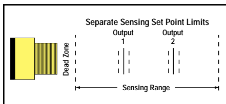
Figure 2b. Programming separate sensing set point limits
