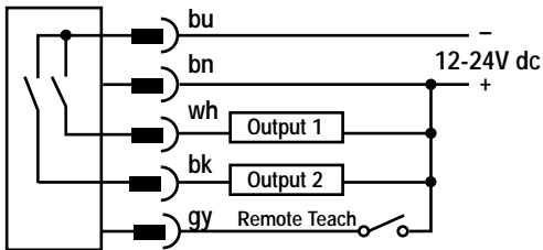
Quick-Disconnect NPN
