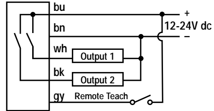
Quick-Disconnect PNP
