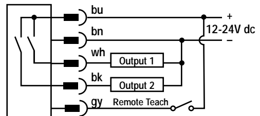
Quick-Disconnect PNP
