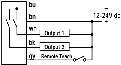
Quick-Disconnect NPN
