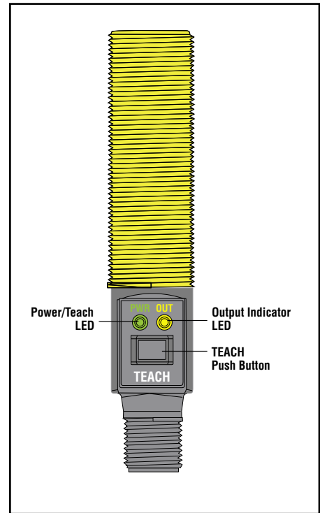
Figure 1. Sensor features
